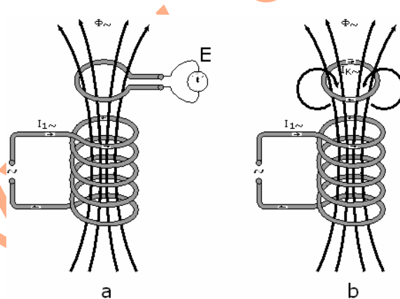
Figure 1: Induction law of Faraday
